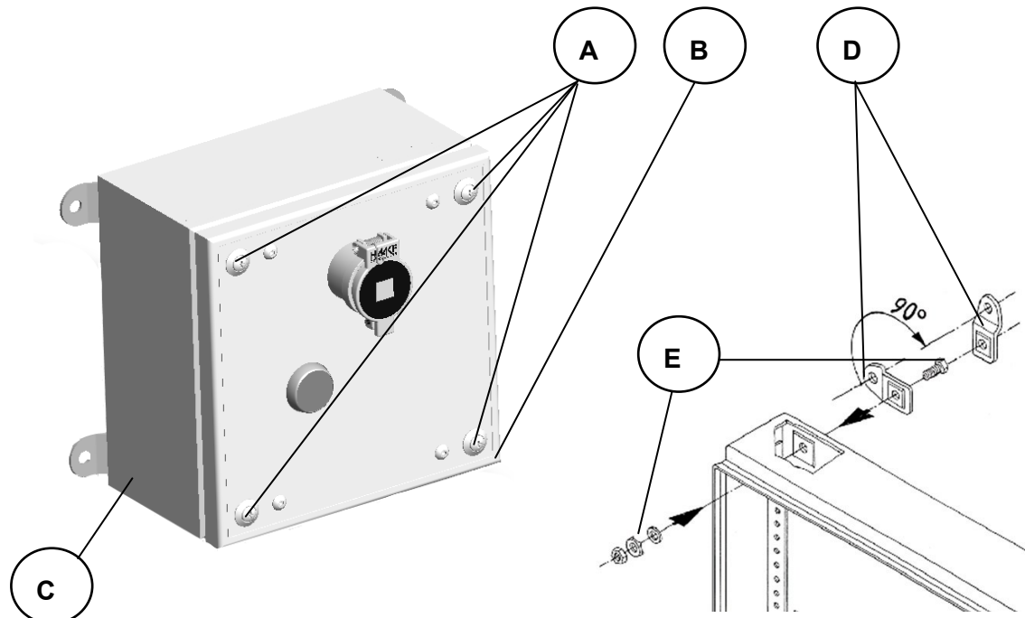
Illustration of HST-M1 Ident. No.: 10219 housing version
