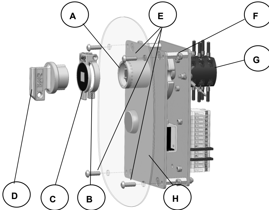
Illustration of HST-M1 Ident. No.: 10213
